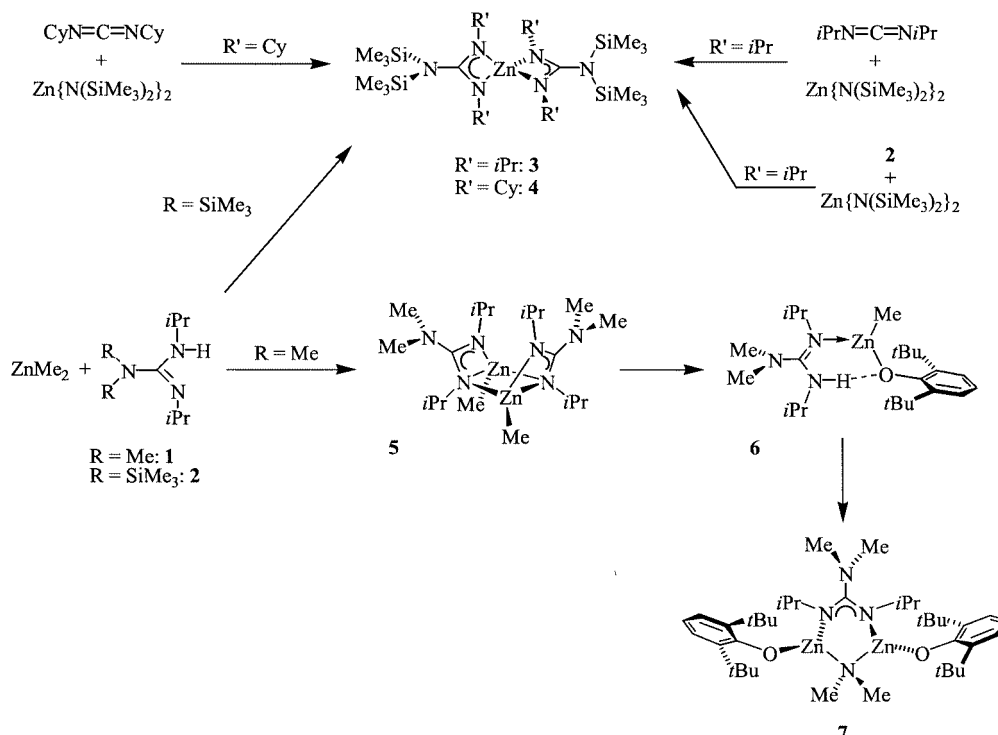
Scheme 1. Summary of the synthesis of zinc guanidinate complexes 3–7
