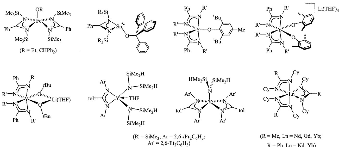
Figure 2. Metal complexes, supported by amidinate ligands, that are active for ring-opening polymerisation
