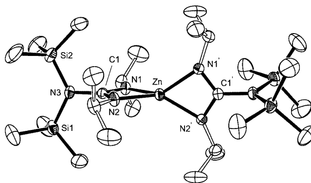
Figure 4. Molecular structure of [Zn\{(Me_3Si)_2NC(NiPr)_2\}_2] ( 3 ) with thermal ellipsoids drawn at the 30% probability level; hydrogen atoms omitted for clarity
