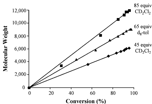
Figure 11. Plot of molecular weight vs. monomer conversion (determined by ^1\text{H} NMR spectroscopy) for the polymerisation of LA with 8
