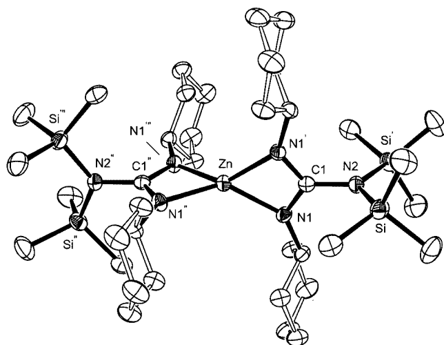
Figure 5. Molecular structure of [\text{Zn}\{(\text{Me}_3\text{Si})_2\text{NC}(\text{NCy})_2\}_2] ( 4 ) with thermal ellipsoids drawn at the 30% probability level; hydrogen atoms omitted for clarity
