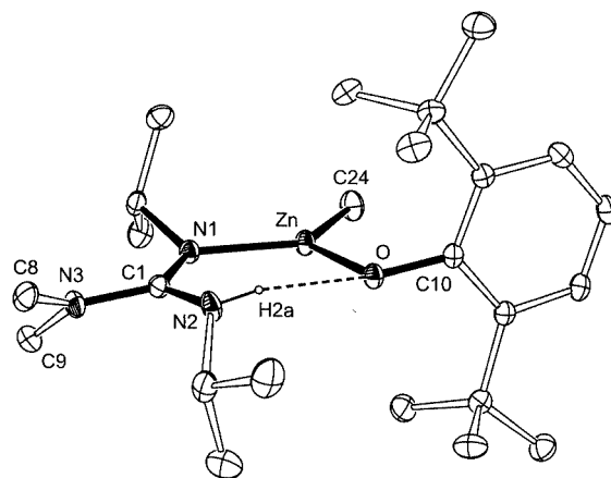
Figure 7. Molecular structure of [\text{Zn}(\text{OAr})\text{Me}\cdot\{\text{Me}_2\text{NC}(\text{N}i\text{Pr})(\text{NH}i\text{Pr})\}] ( 6 ) with thermal ellipsoids drawn at the 30% probability level; hydrogen atoms, except \text{H}(2a) , omitted for clarity
