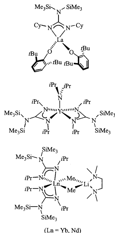
Figure 3. Metal complexes, supported by guanidinate ligands, that are active for ring-opening polymerisation
