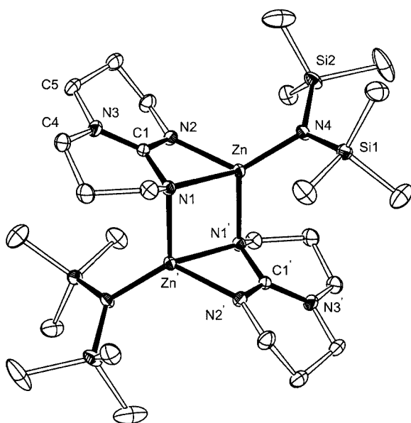
Figure 10. Molecular structure of [\text{Zn}(\text{hpp})\{\text{N}(\text{SiMe}_3)_2\}_2] ( 8 ) with thermal ellipsoids drawn at the 30% probability level; hydrogen atoms omitted for clarity
