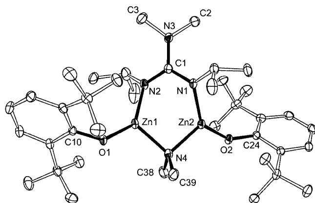
Figure 8. Molecular structure of [\{\text{Zn}(\text{OAr})\}_2(\mu\text{-}\{\text{Me}_2\text{NC}(\text{N}i\text{Pr})_2\})(\mu\text{-NMe}_2)] ( 7 ) with thermal ellipsoids drawn at the 20% probability level; hydrogen atoms omitted for clarity
