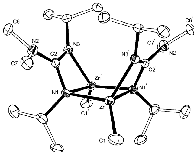
Figure 6. Molecular structure of [\text{Zn}\{\text{Me}_2\text{NC}(\text{NiPr})_2\}\text{Me}]_2 ( 5 ) with thermal ellipsoids drawn at the 30% probability level; hydrogen atoms omitted for clarity
