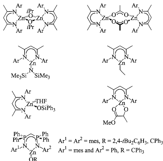
Figure 1. Zinc complexes, supported by \beta -diketiminate and related ligands, that are active for the ring-opening polymerisation of lactide
