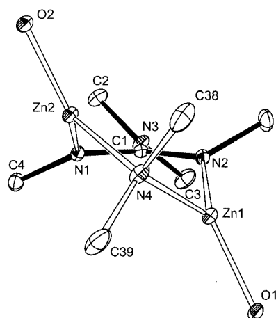
Figure 9. Core of [\{\text{Zn}(\text{OAr})\}_2(\mu\text{-}\{\text{Me}_2\text{NC}(\text{N}i\text{Pr})_2\})(\mu\text{-NMe}_2)] ( 7 ) along the approximate N(4)–C(1)–N(3) vector, illustrating the “half-chair” geometry of the metallacycle, and the distribution of the ligand substituents
